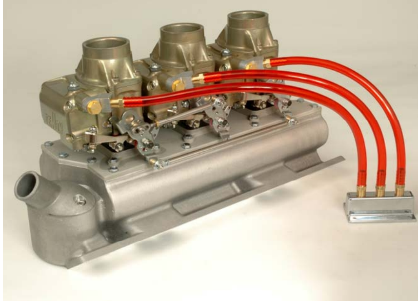
Part # 9808 shown, shipped complete with fuel lines and fuel block
